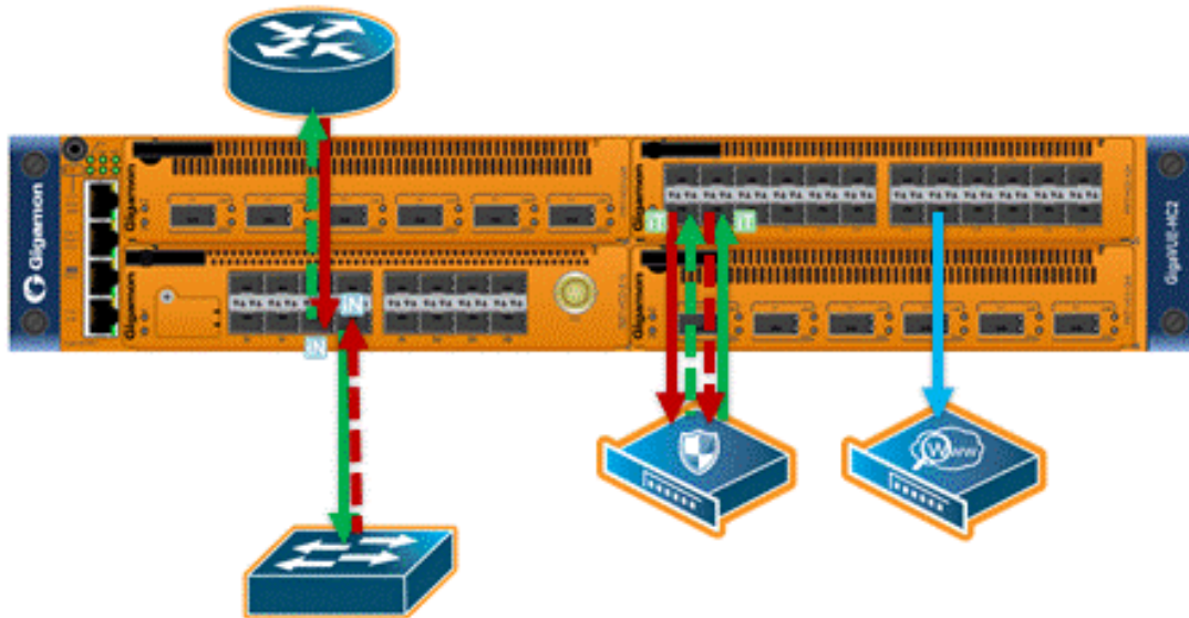
Figure 11 Logical Bypass
